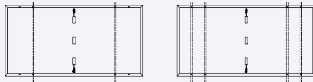
Figure 12-2: Mounting rails must run perpendicularly to the long frame (120 or 144 cell modules)
